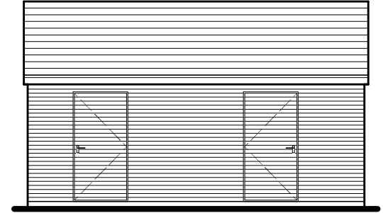
L/H ELEVATION SCALE - 1:100
