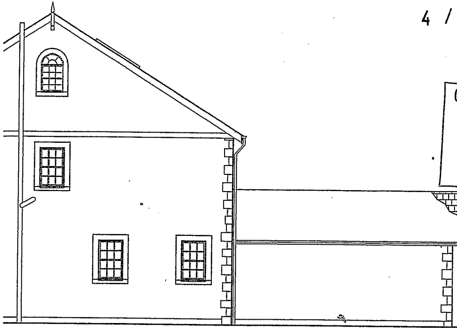
Side elevation View A - A (1st. angle)
